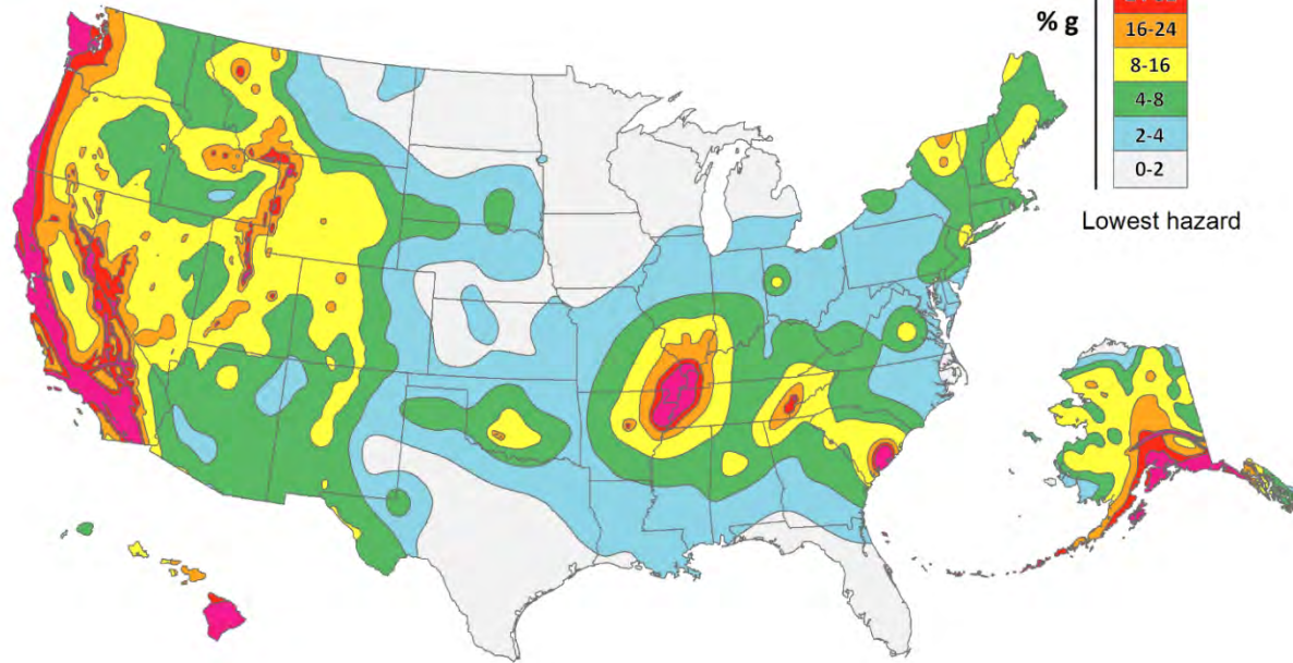
Figure 4-40: United States Earthquake Hazard Map
