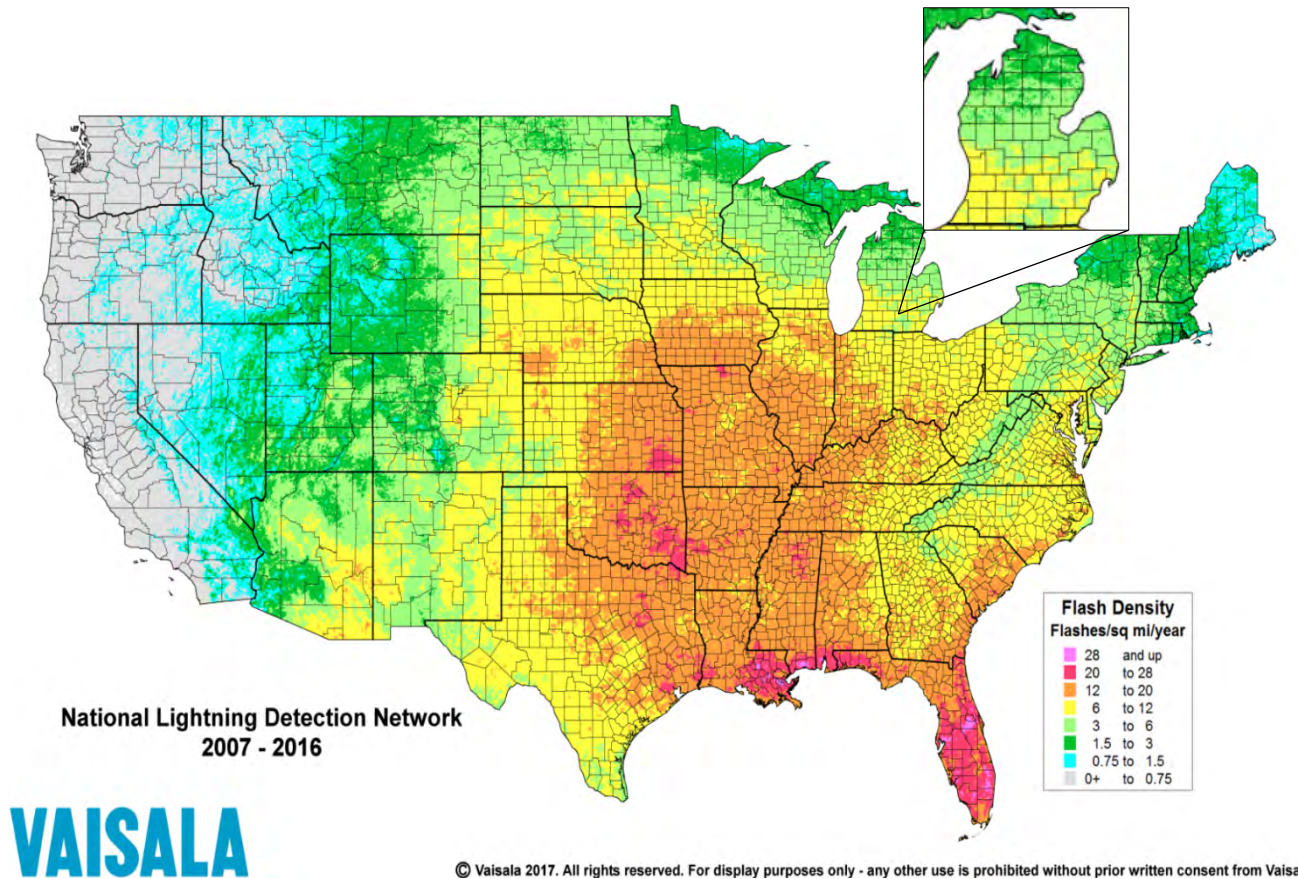
Figure 4-11: Vaisala, Inc. Average Lightning Flash per Square Mile (2007-2016)
