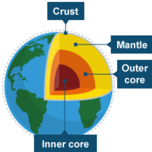
Figure 4-38: Earth's Sub Layers
