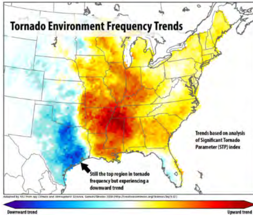
Figure 4-17: U.S. Tornado Frequency Shifting Eastward
