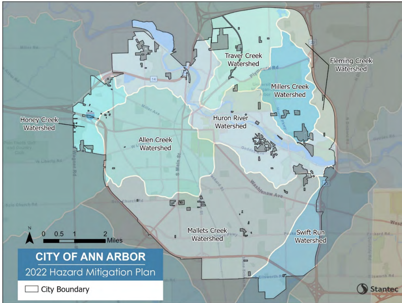
Figure 4-20: Ann Arbor Watersheds
