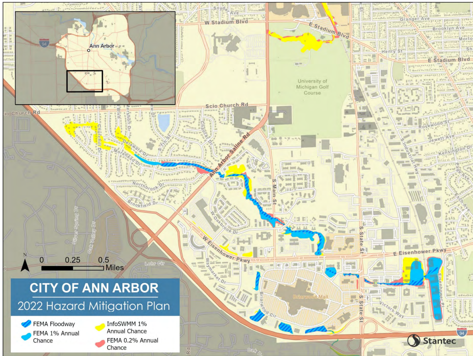
Figure 4-24: Ann Arbor InfoSWMM Model Comparison – Malletts Creek West of South Seventh Street
