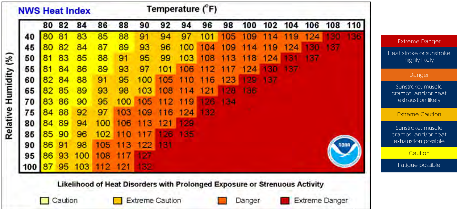
Figure 4-6: National Weather Service Heat Index Chart
