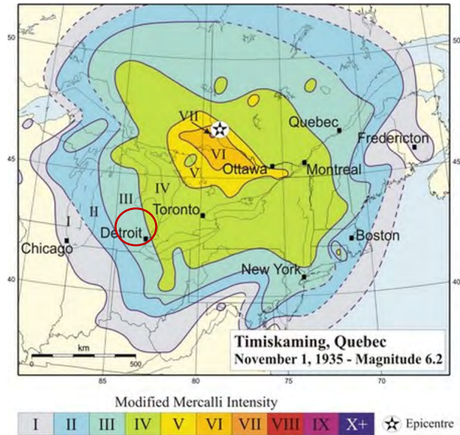
Figure 4-43: 1935 Timiskaming Earthquake Map
