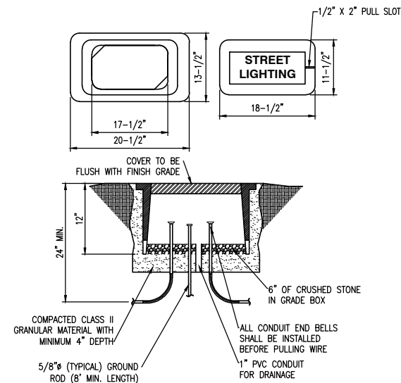
HANDHOLE DETAIL
