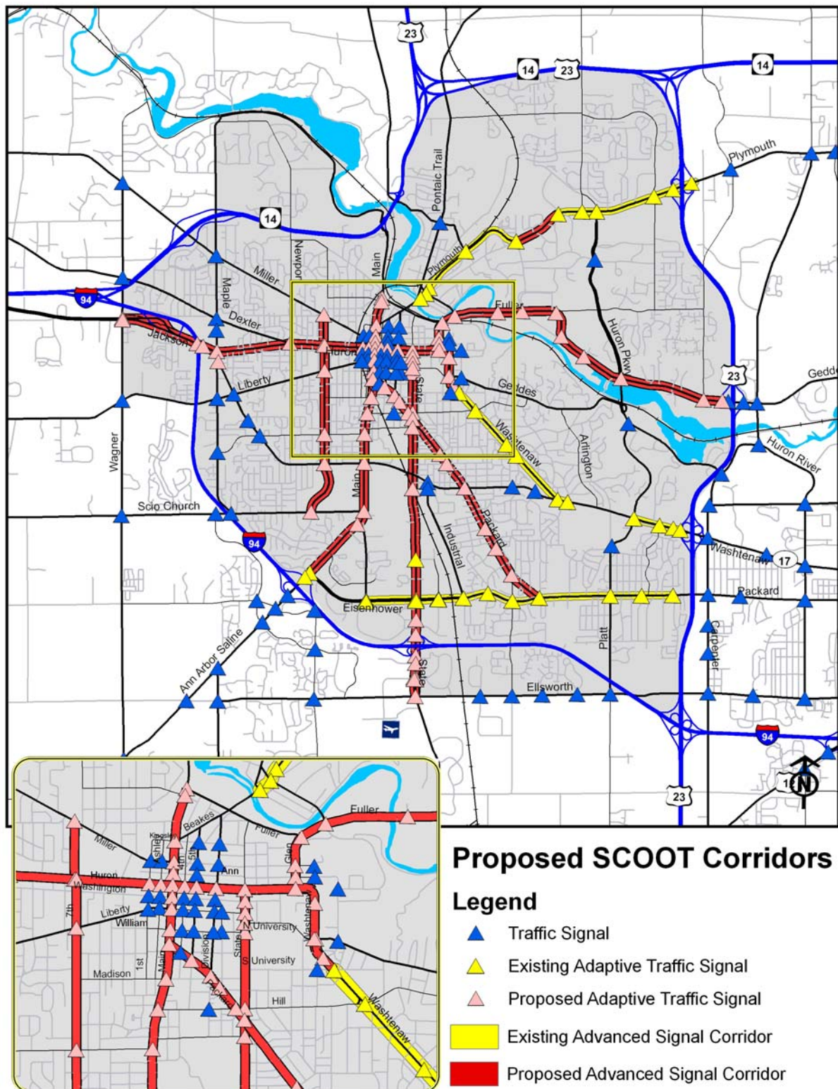
Figure 6-3: Existing and Proposed SCOOT Expansion Locations
