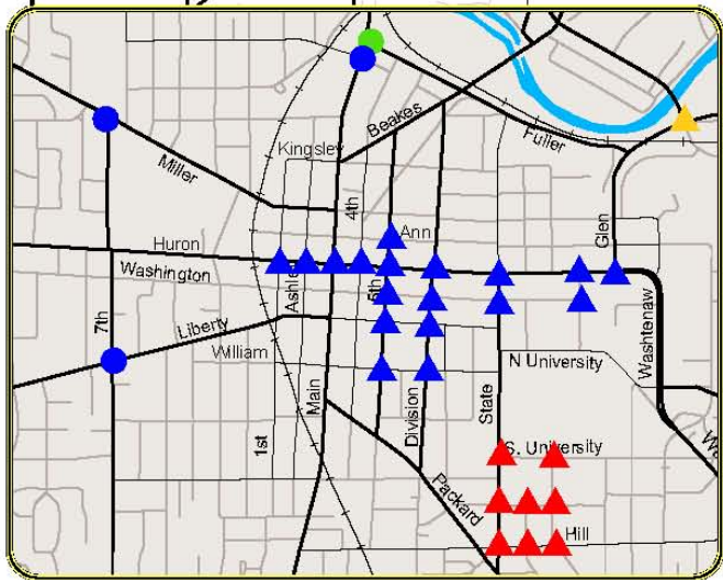
Figure 4-4: Ann Arbor Existing Conditions Intersection 2008 Levels of Service-PM Peak Hour
