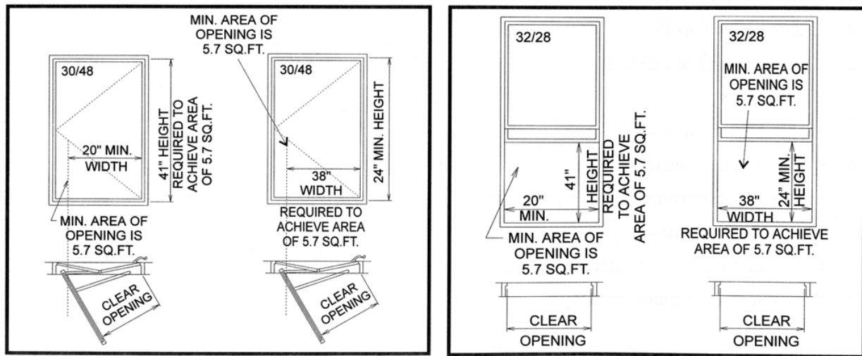
Casement
