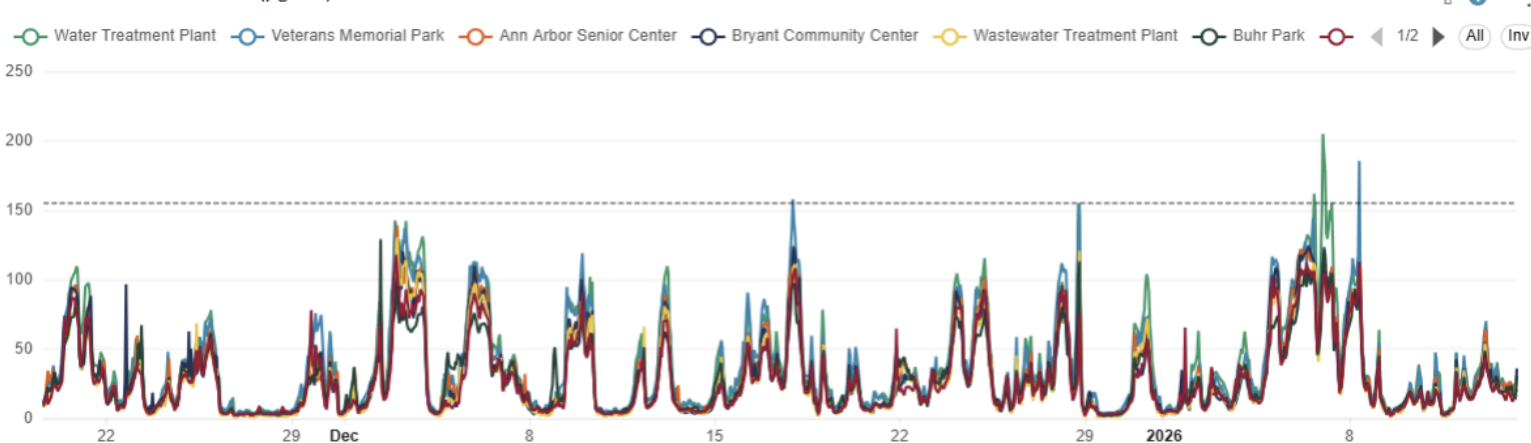
Particulate Matter <10 microns (µg/m3)
