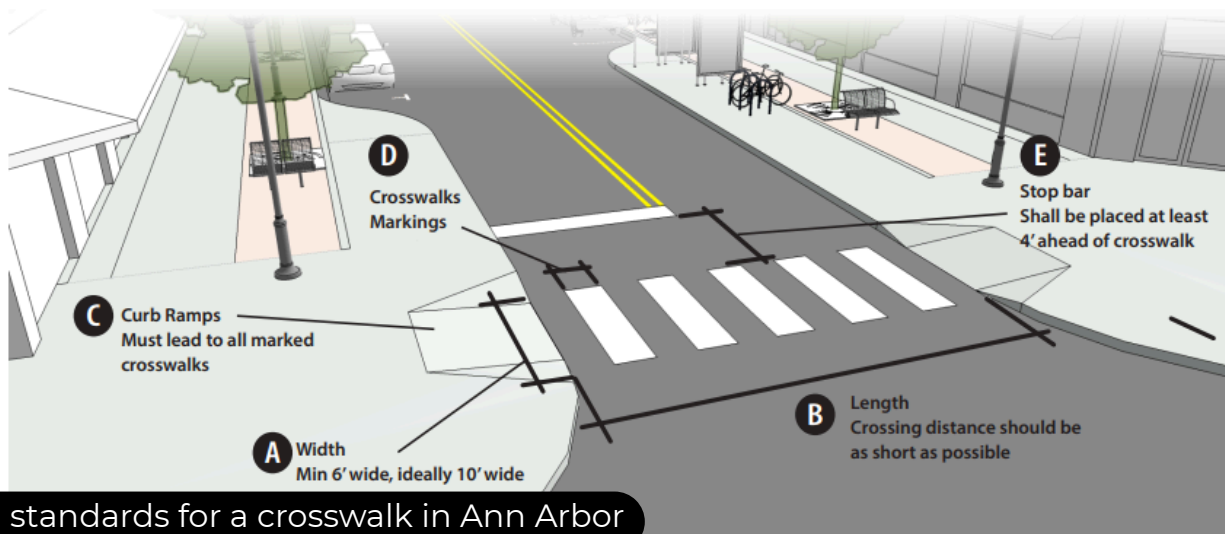
Figure 4.1.3 - Crosswalks
