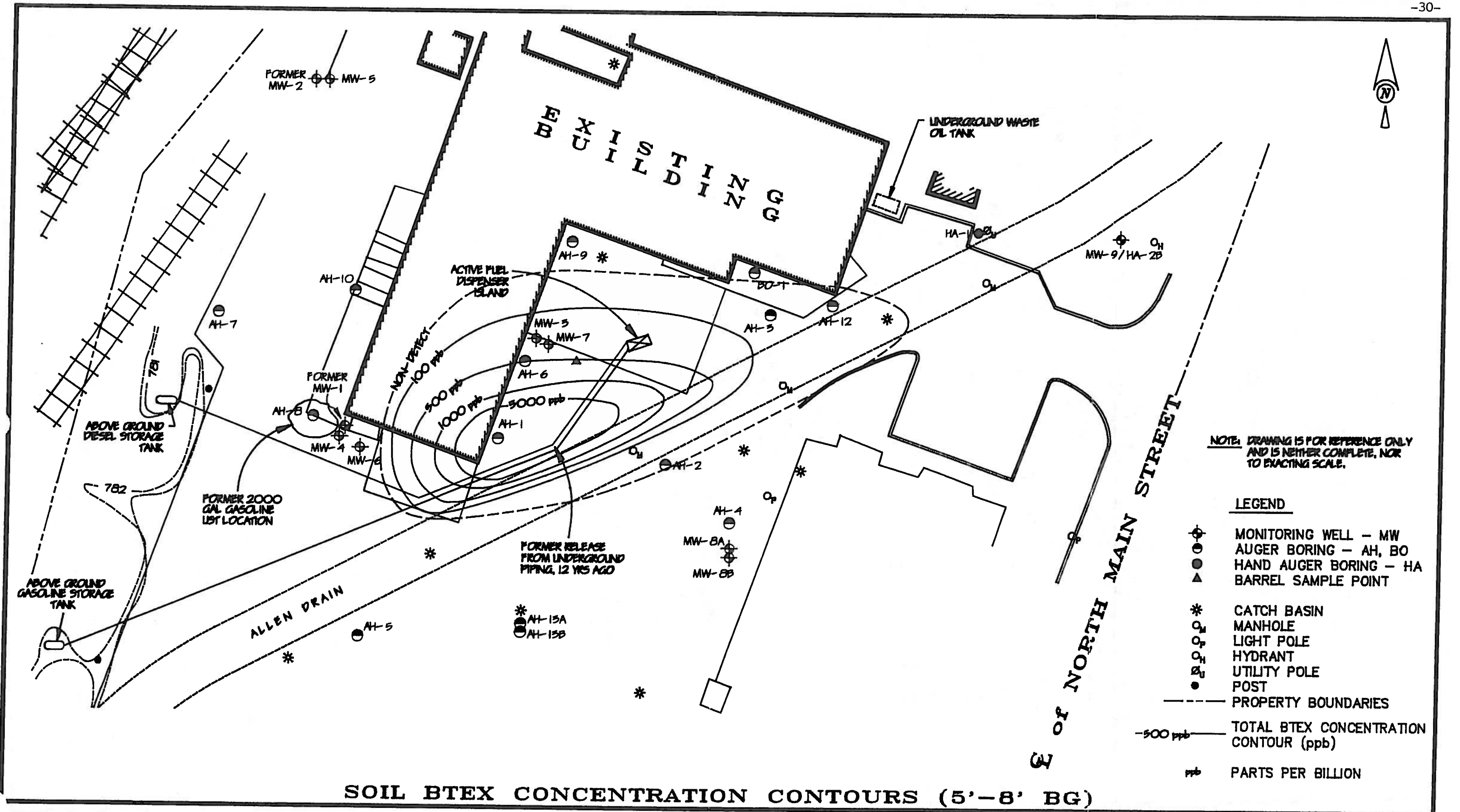
FIGURE 5 - SOIL BTEX CONCENTRATION CONTOURS (5'-8' BELOW GRADE) CITY OF ANN ARBOR CITY MAINTENANCE GARAGE 721 N. MAIN ST., ANN ARBOR, MI 05/28/93 EPH CAA90087
