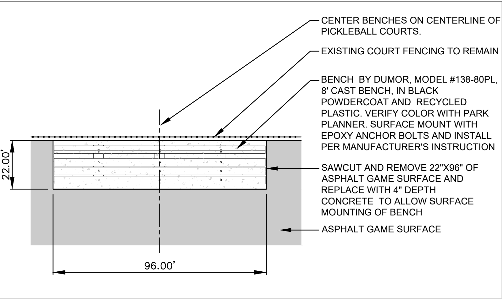
PLAN VIEW
