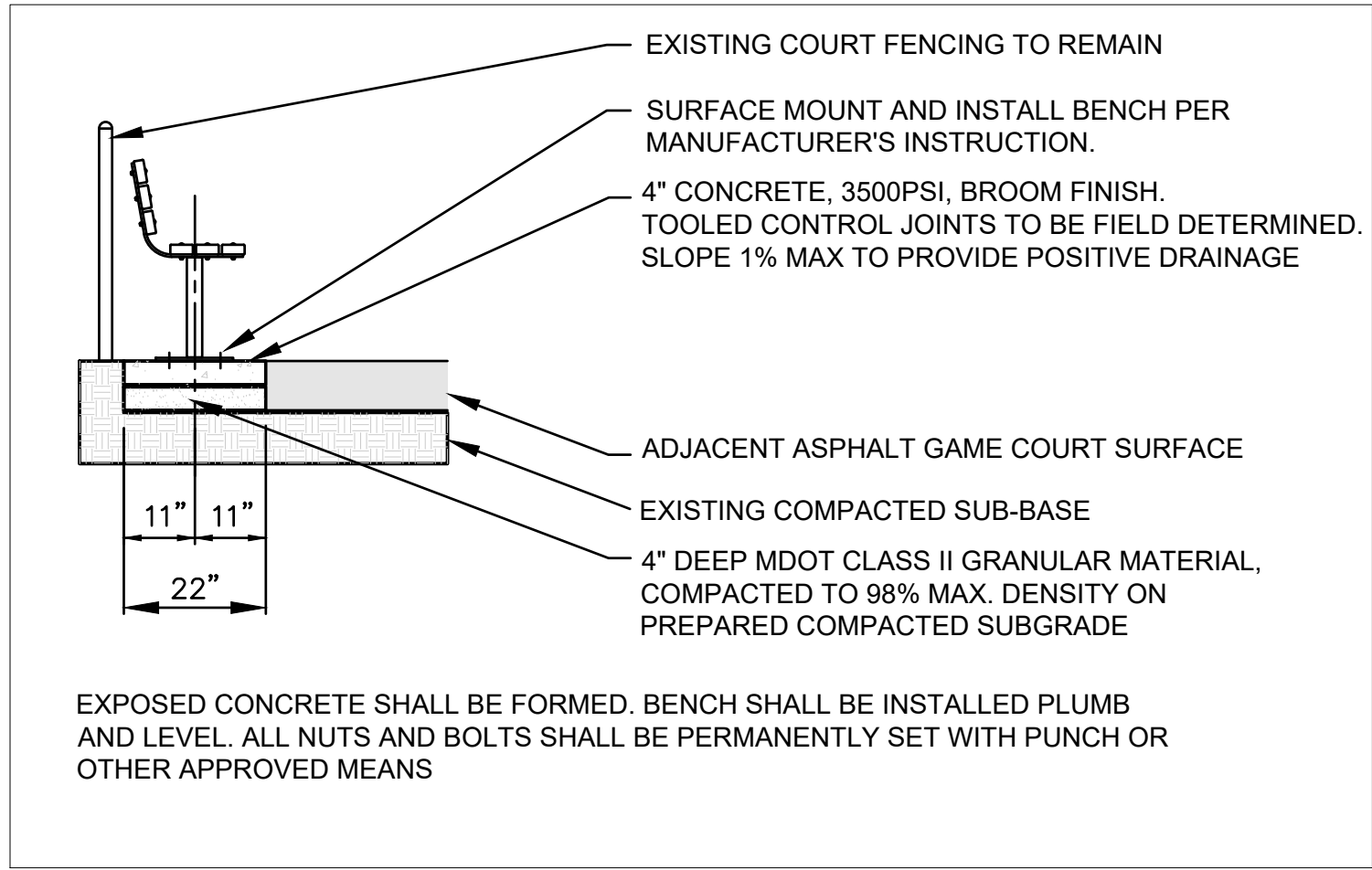
SECTION VIEW
