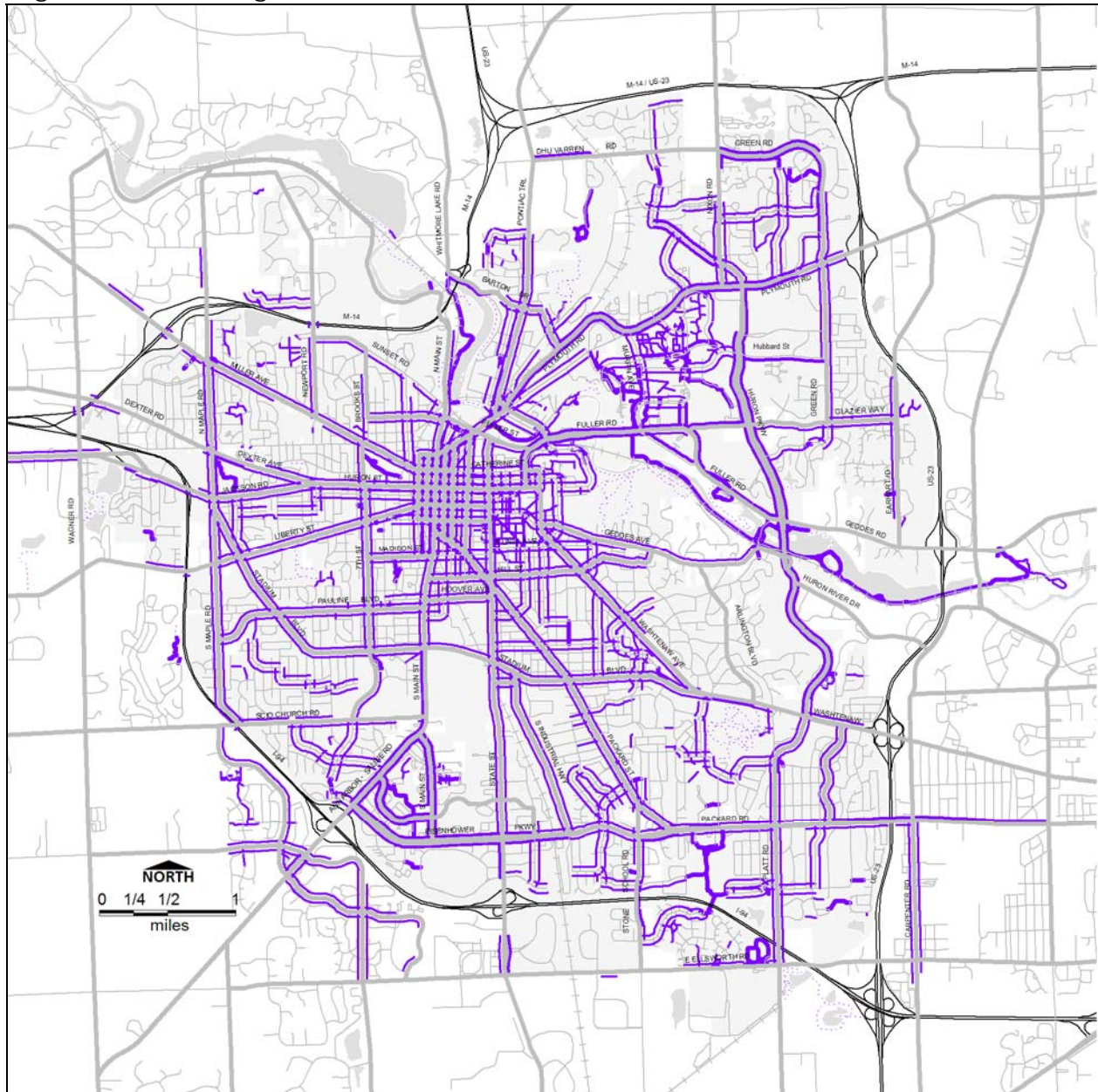
Fig. 4.2A. Existing Pedestrian Facilities
