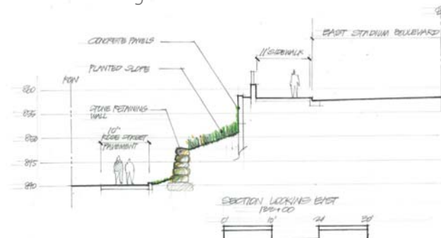
Section Along Rose Avenue
