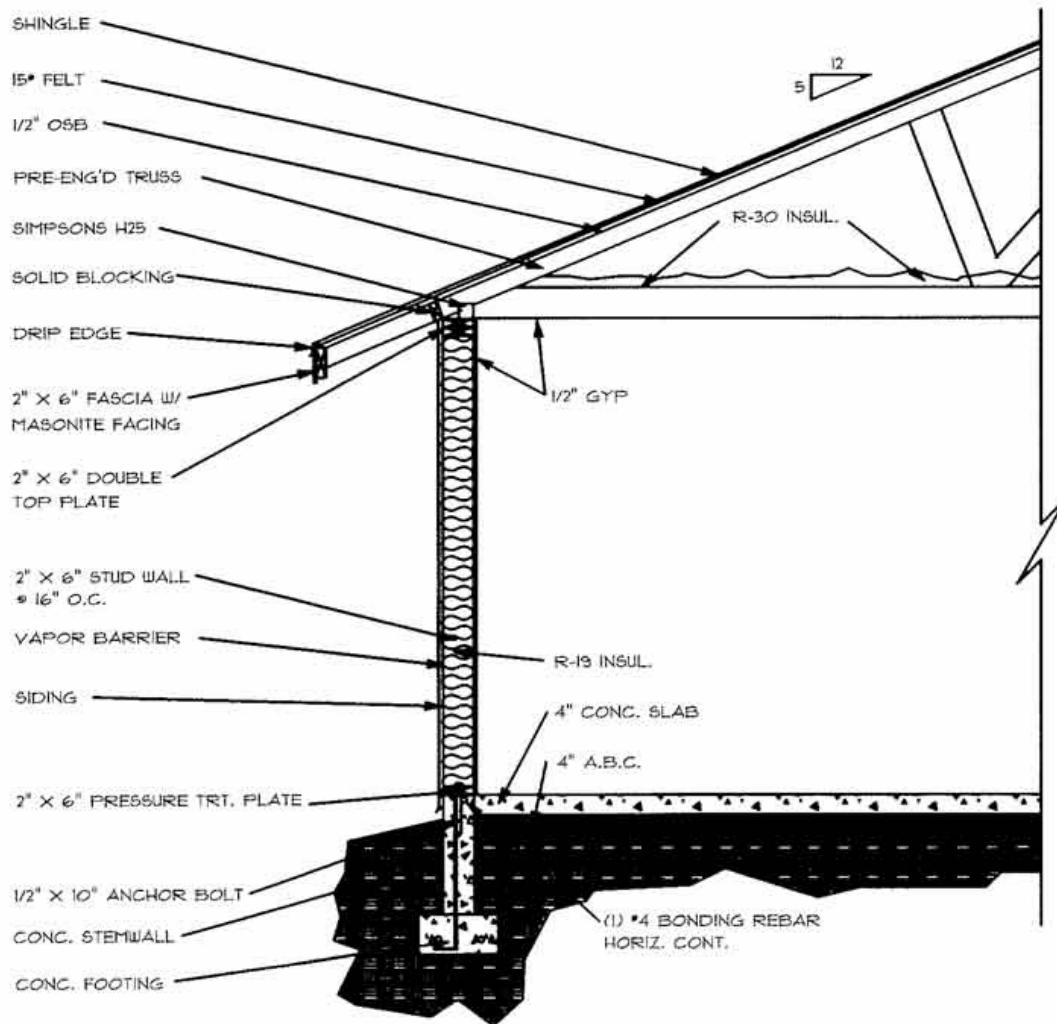
2" X 6" WALL SECTION
